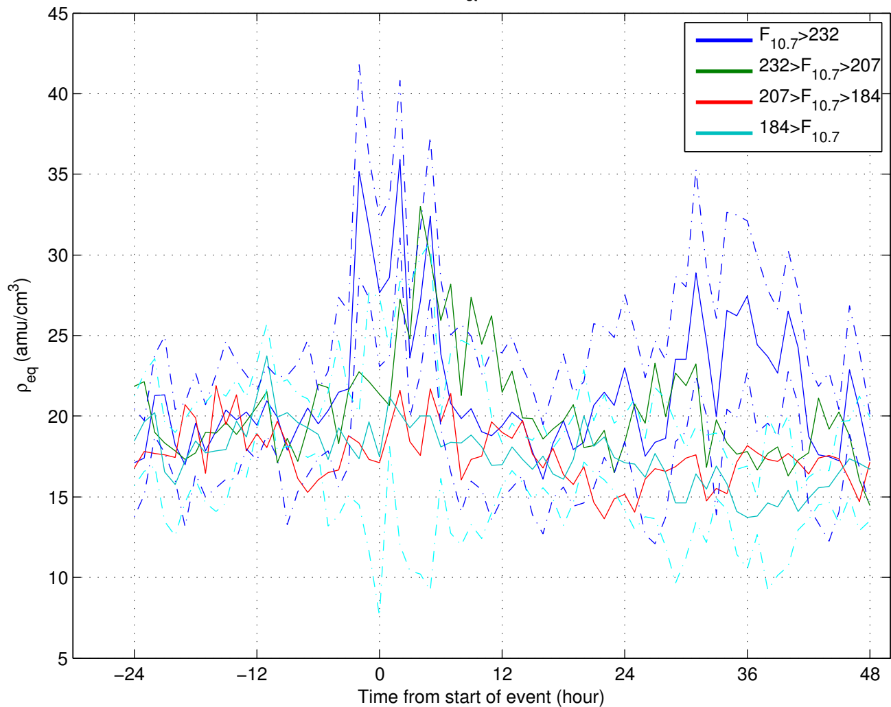
355 evenly-binned events of D_{st} < -50 (nT) for GOES6: 1989–1991
